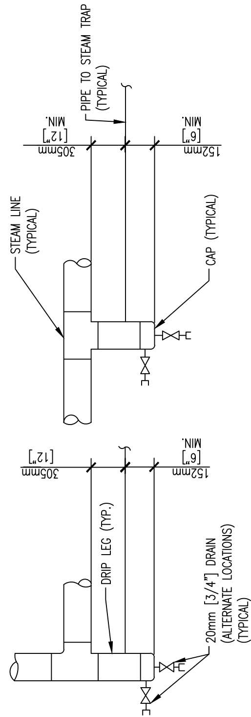
STEAM LINE DRIP POCKET
